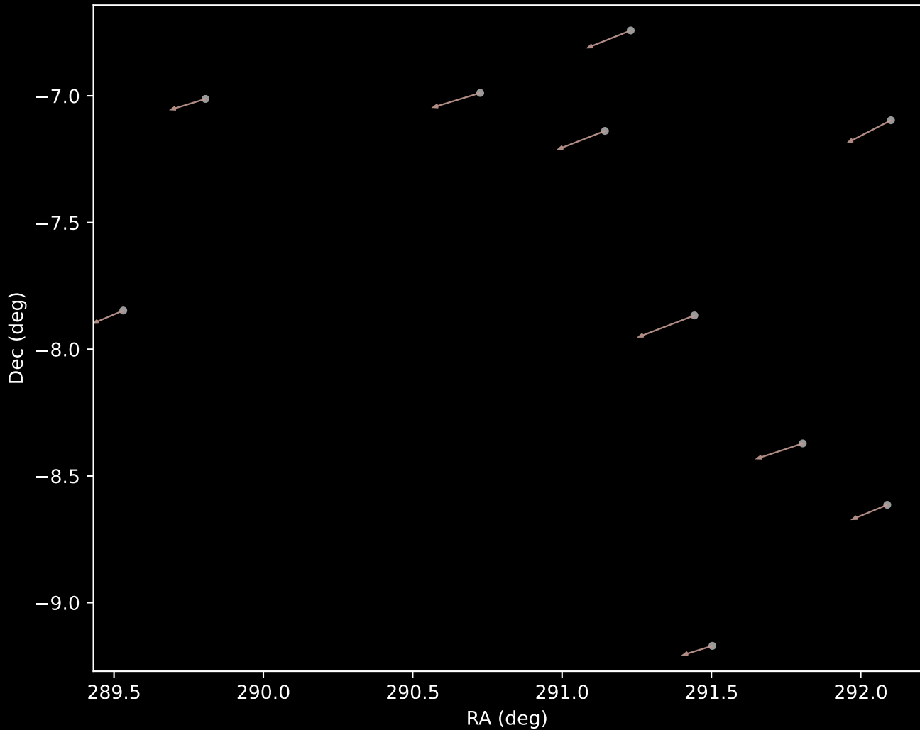
APOGEE DR17 Cluster 11 Proper Motion Vectors (n=10)
