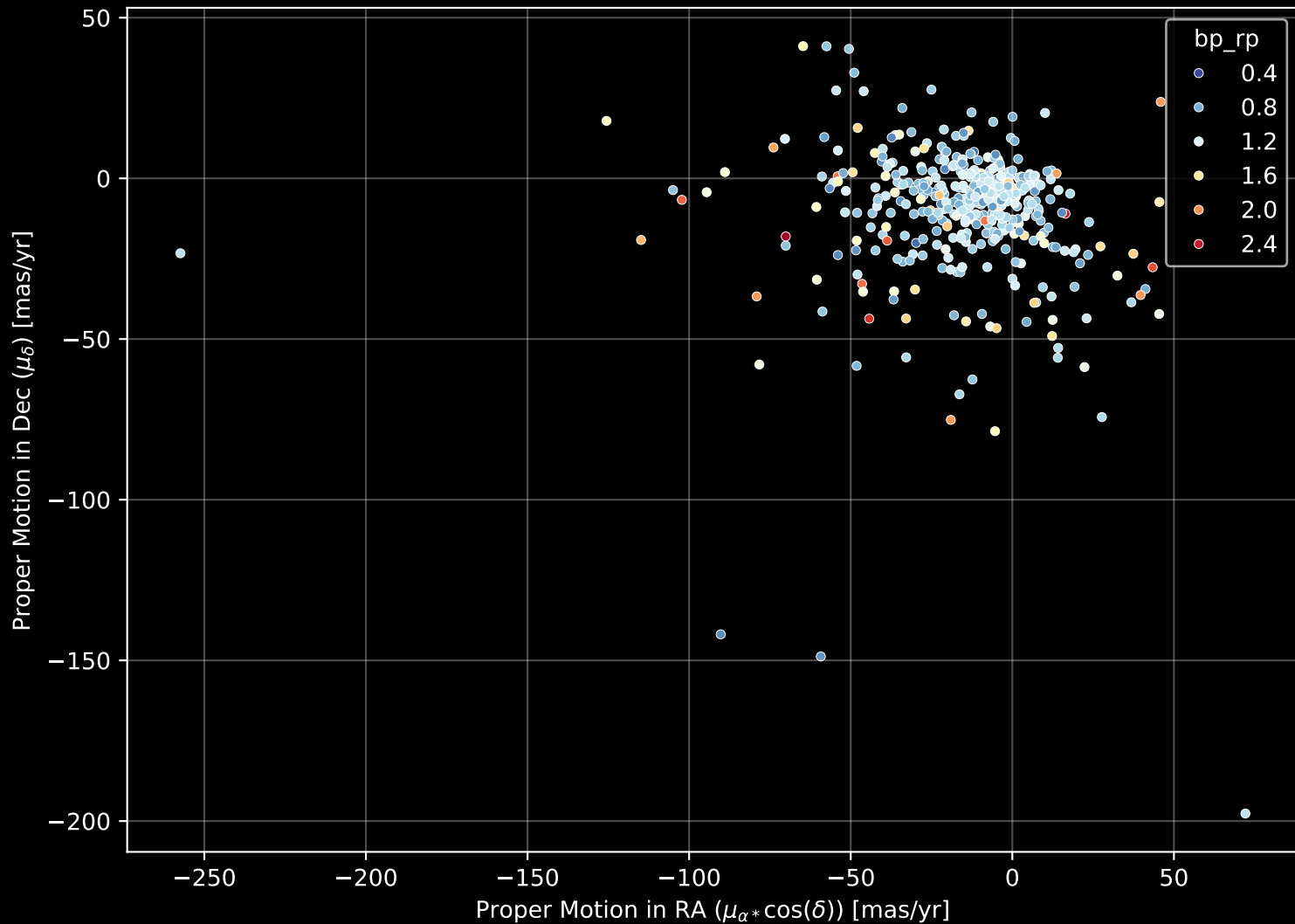
APOGEE DR17 Field: [VOD3] Proper Motion Diagram (n= 489)
