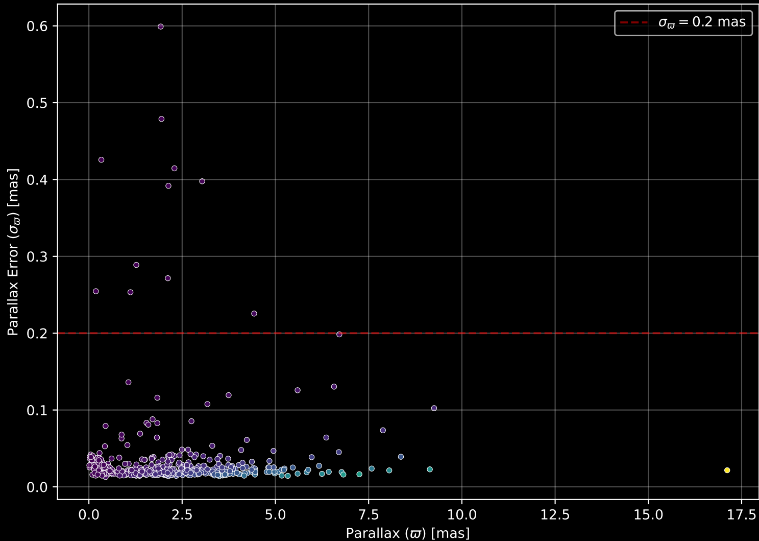
APOGEE DR17 Field: [VOD3] Parallax Quality (n= 489)
