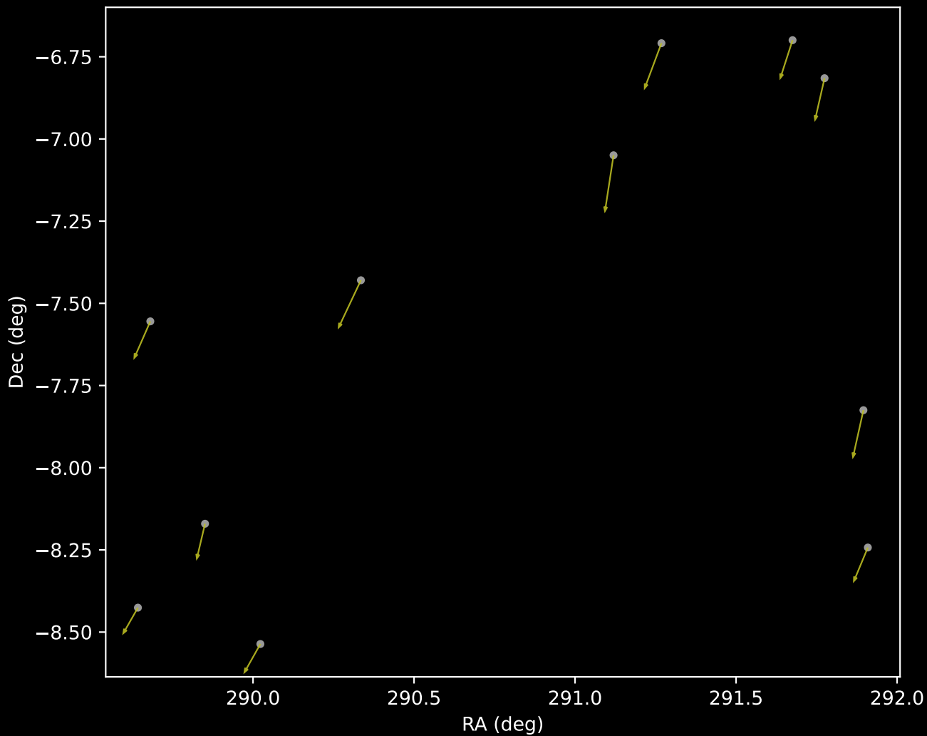
APOGEE DR17 Cluster 16 Proper Motion Vectors (n=11)
