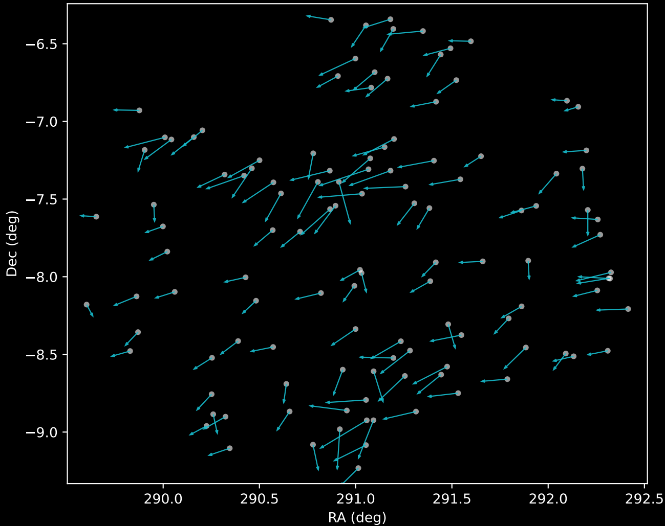
APOGEE DR17 Cluster 18 Proper Motion Vectors (n=119)
