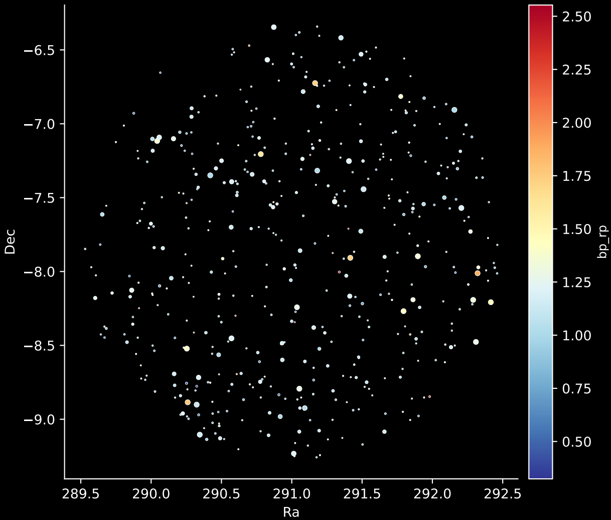
APOGEE DR17 Field: [VOD3] Stars: 489
