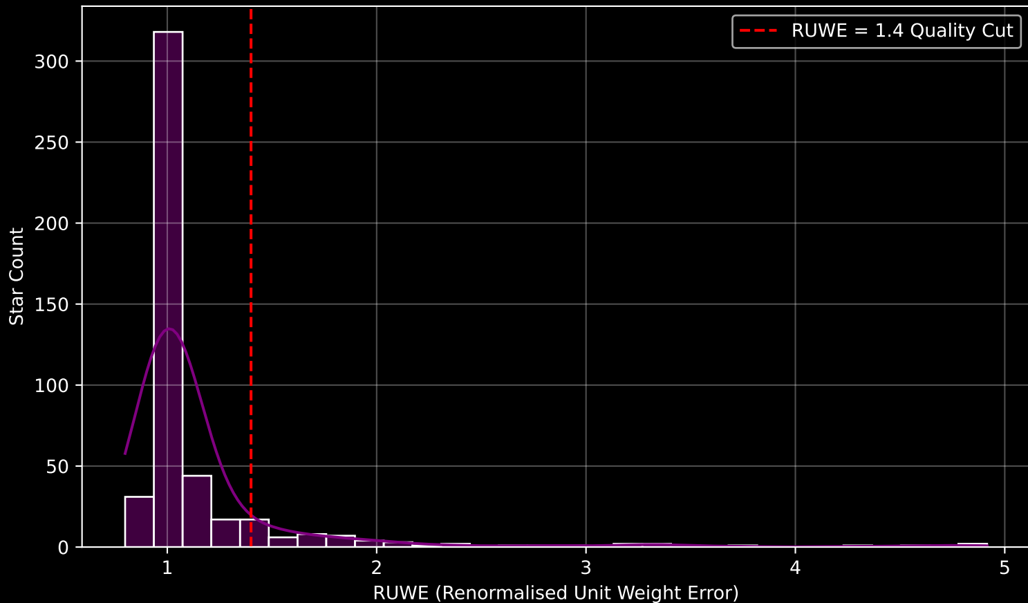
GAPOGEE DR17 Field [VOD3] RUWE Distribution (n= 472)
