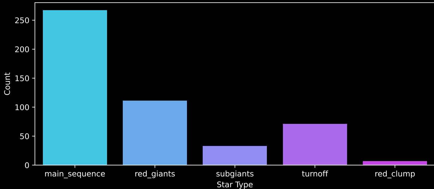
APOGEE DR17 Field: [VOD3] Count plot of Star Type
